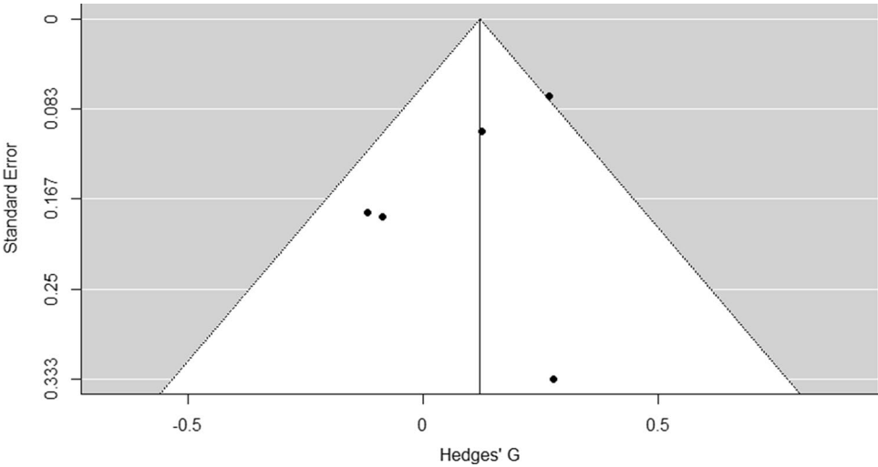
Fig. 3 Funnel plot (standard error vs. Hedges' G ) for studies meeting inclusion criteria
