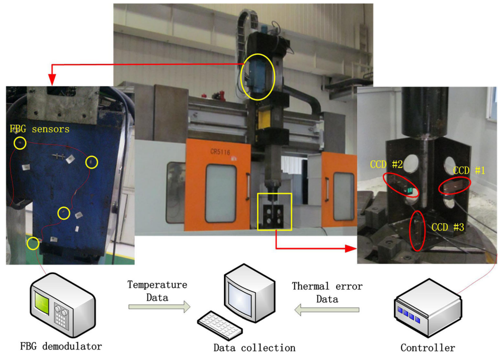
Fig. 4 Temperature and thermal error collection system
