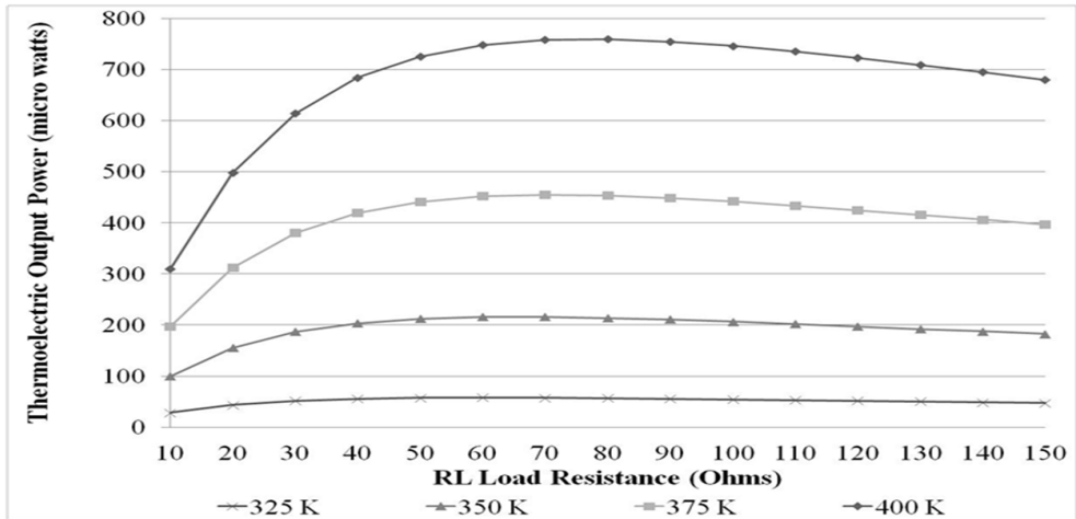
Figure 12. The electrical power generated at the load resistor (RL) with a doping concentration of 1e^{16}cm^{-3} and different temperature settings applied to the thermal contacts Copper 1, Copper 4 and Copper 6 [8]
