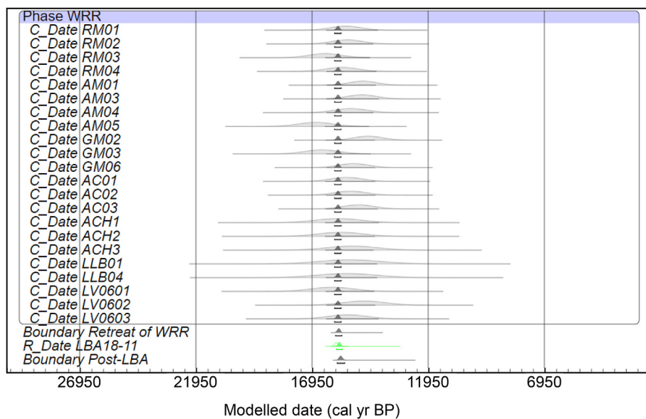
Fig. 6. Probability distribution functions of the recalibrated WRR TCN ages as well as our new age from Loch Ba na h-Achlaise as produced by our OxCal model (see Fig. S7 for the full model output).
