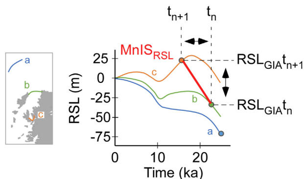
Fig. 2. Conceptual model showing how rates of sea-level by the Minch Ice Stream ice front were determined. Top row panels illustrate GIA predicted rates of RSL change from 27–10 ka at three locations of the Minch Ice Stream ice front, a, b, and c. The bottom row shows how RSL_{MnIS} is calculated from the GIA predictions at t_0 , t_n , and t_{n+1} . See text for details.
