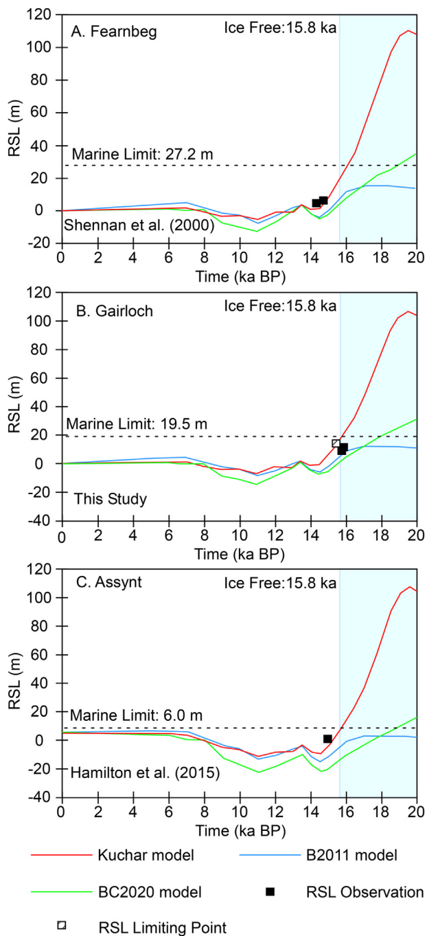
Fig. 7. Comparison of RSL observations to three GIA model predictions for A.) Fearnbeg, B.) Gairloch (including both Loch Bad na h-Achlaise and Glac Bhudhe), and C.) Assynt. See Fig. 1 for geographic locations. RSL observations for A and C are from (Shennan et al., 2000) and Hamilton et al. (2015), respectively, while those for B are from this study. The marine limits for A are from Sissons (1977) and Dawson (2009) , while those from B are from Sissons and Dawson (1981) and those from C are from Shennan et al. (2000) and Hamilton et al. (2015) .
