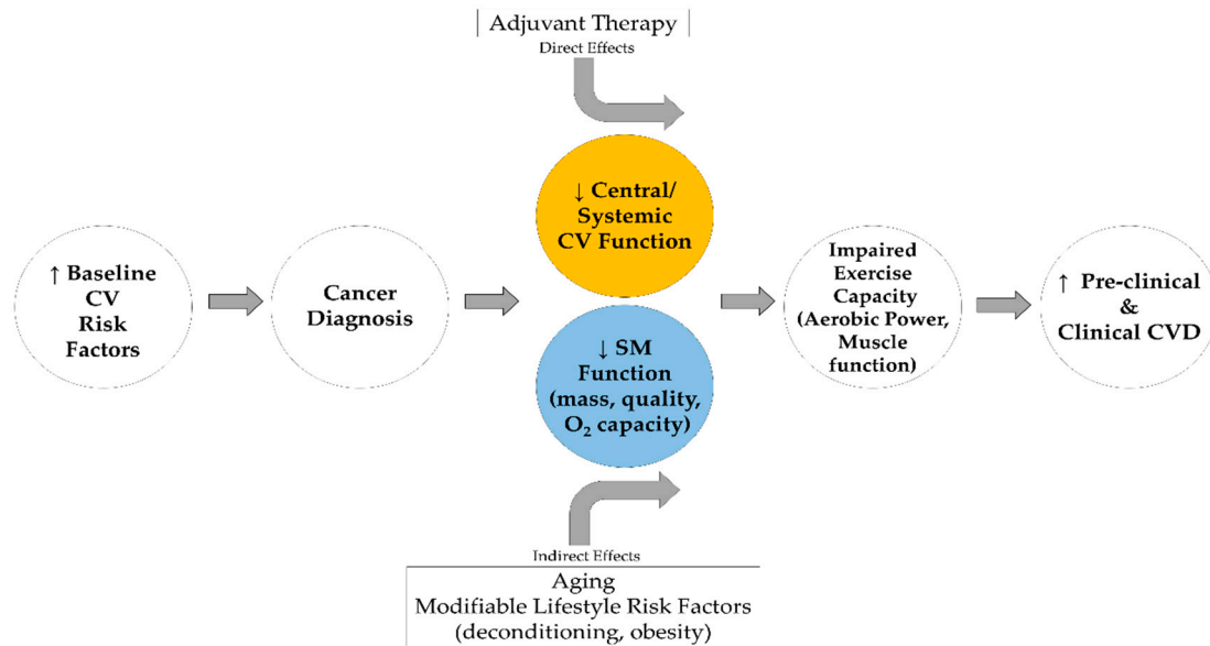
Figure 1. Extended “Multi-Hit” Hypothesis model adapted from Lee Jones et al. (2007). CV, Cardiovascular; O 2 , Oxidative; SM, Skeletal muscle.
