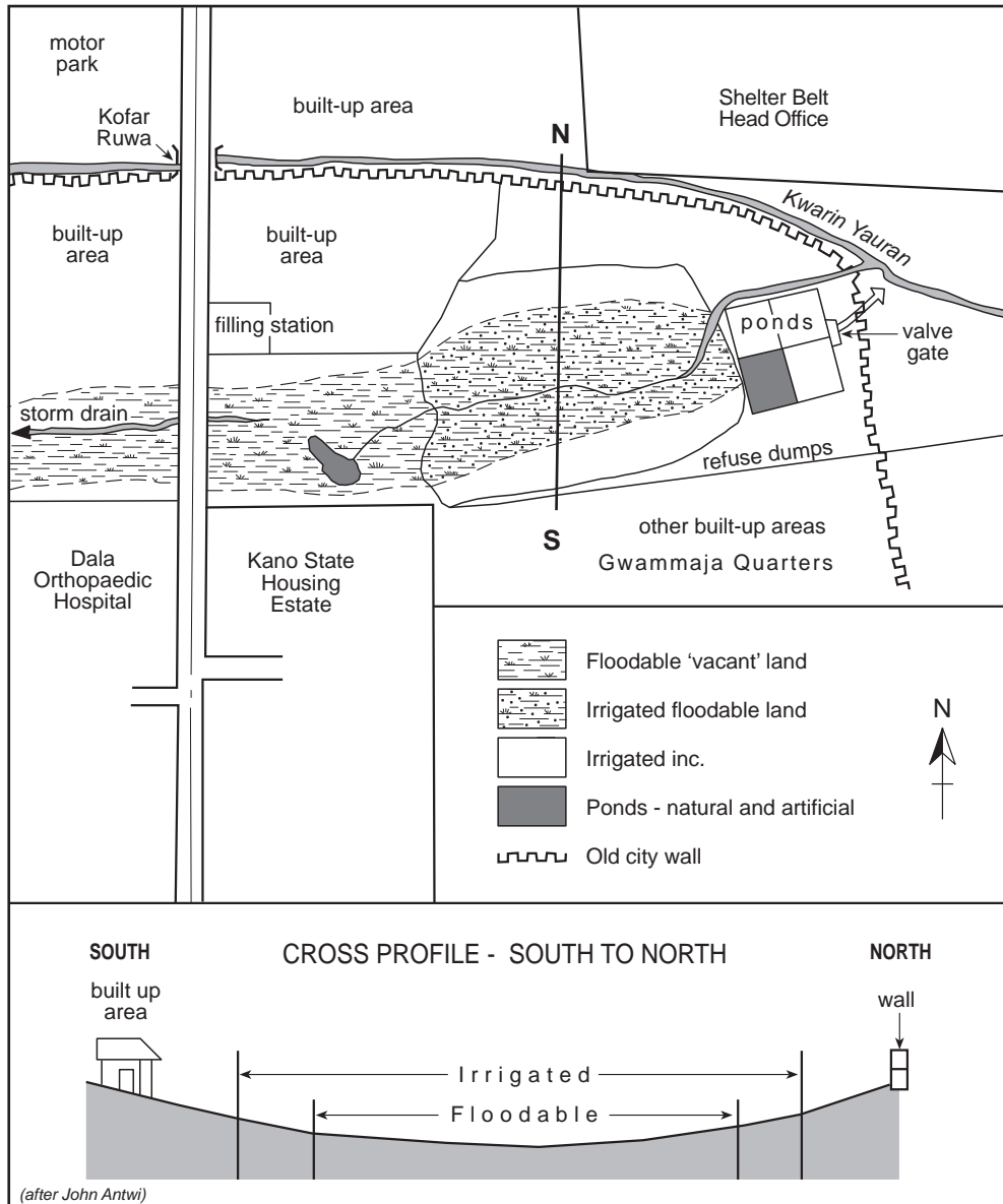
Sketch Map and Cross-section of the Kofar Ruwa Production Site
